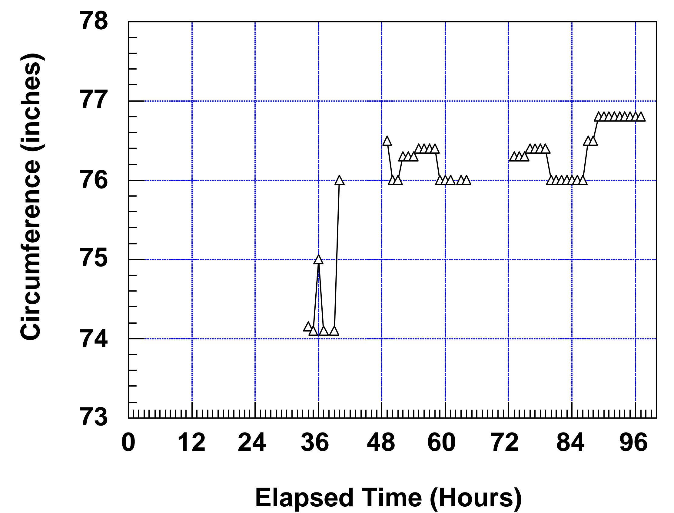
Tree 3 Evapotranspiration Study 6 AM 22 July 2002 - 11 AM 24 July 2002
